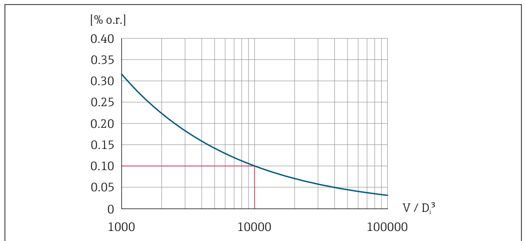
12 Repeatability = 0.1 % o.r. with a measured volume [m³] of V = 10 000 · D i 3
